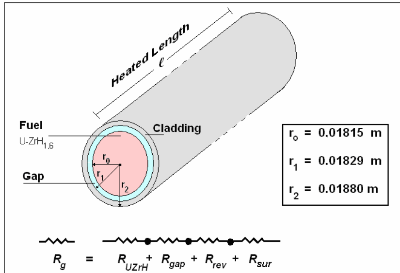
FIG. 6. Fuel element configuration
